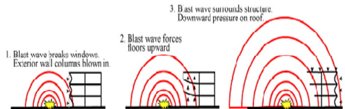
Figure 7. Sequence of air-blast effects [5]
