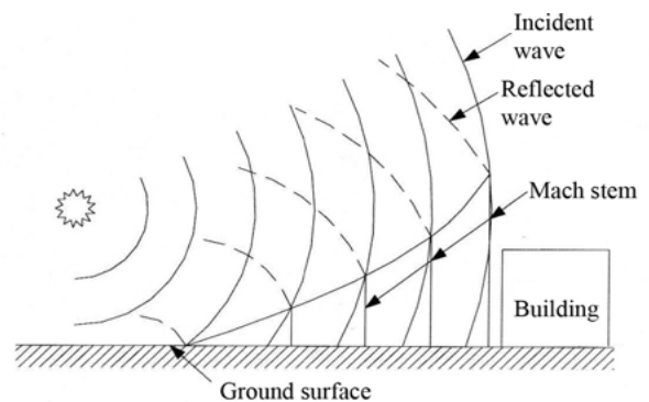
Figure 1. Air burst with ground reflections
