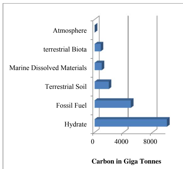
The bar graph compares the carbon in hydrates with the sources of other global carbon cycle
