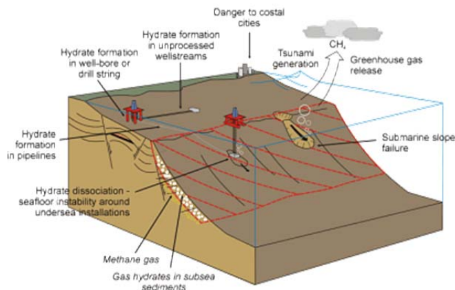
Figure explains the faults while extracting gas. This describes landslide disaster
