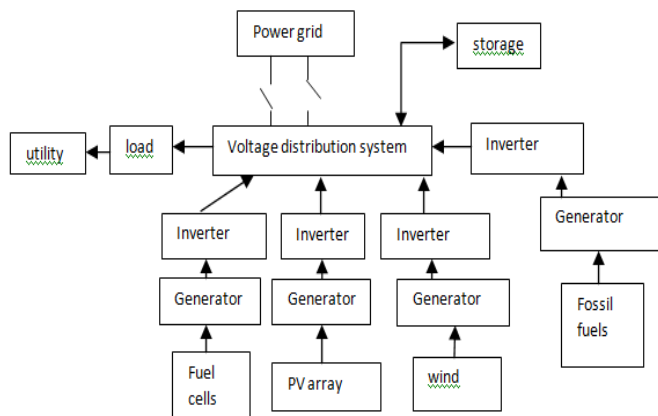
Fig.1 shows the basic block diagram of MICROGRID
