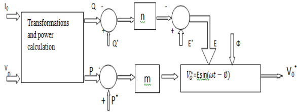
Fig.5 shows the droop control using P/Q Indian scenario on the micro grid
