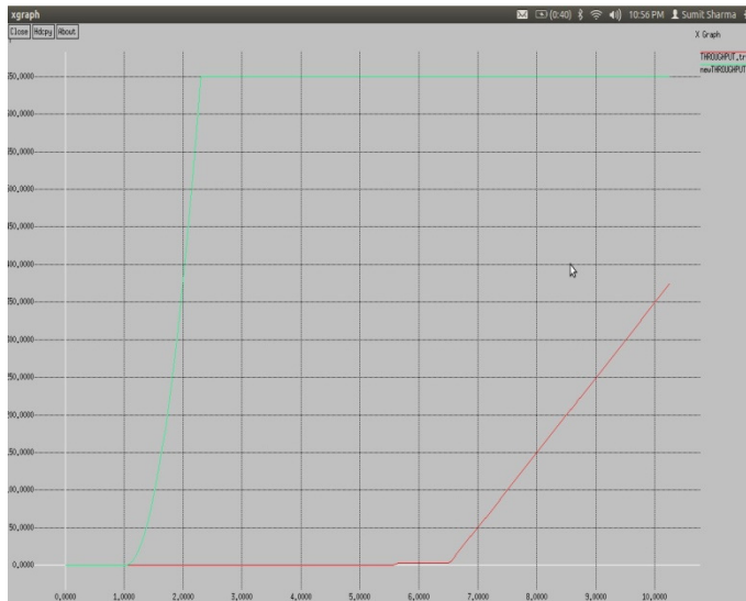
Fig4: Comparison graphs of Throughput
